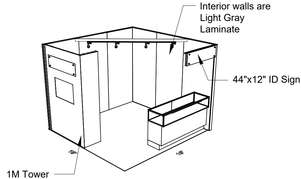
PERSPECTIVE - FRONT
