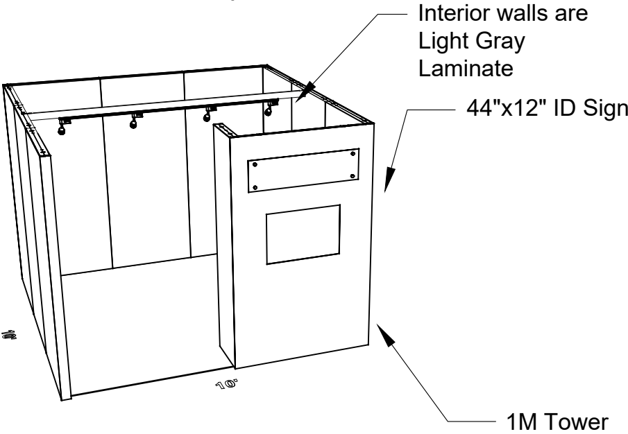
PERSPECTIVE - FRONT
