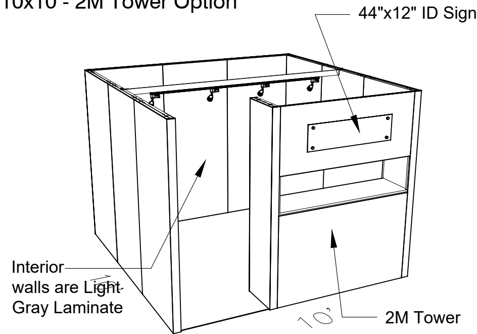
PERSPECTIVE - FRONT
