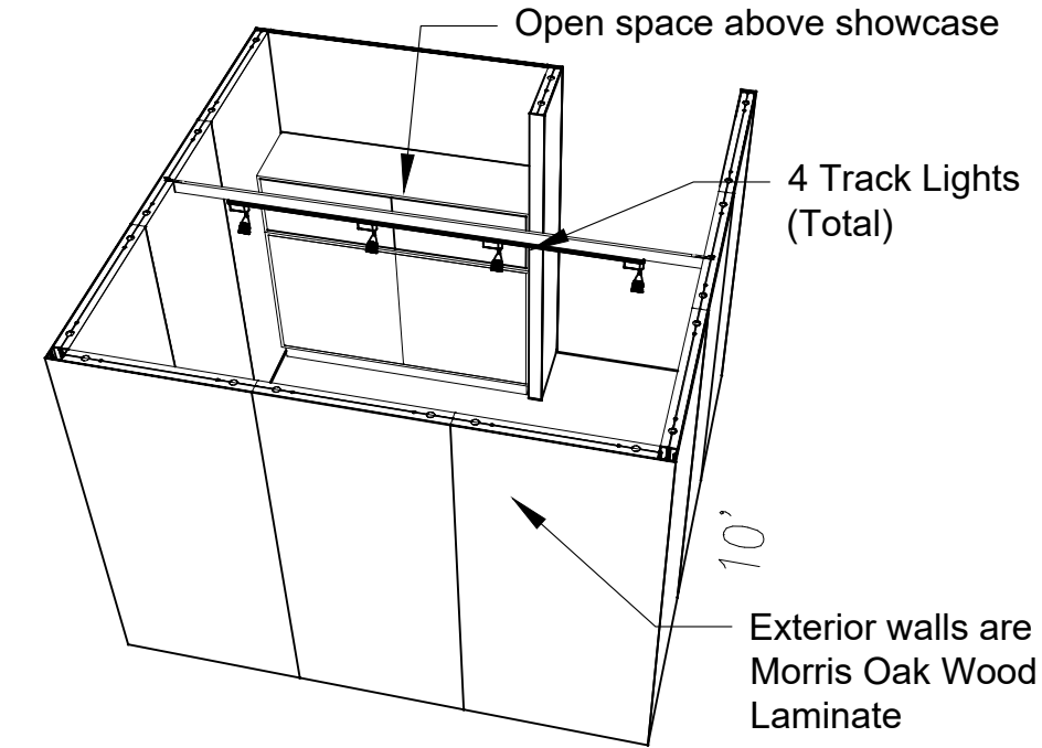
PERSPECTIVE - BACK
