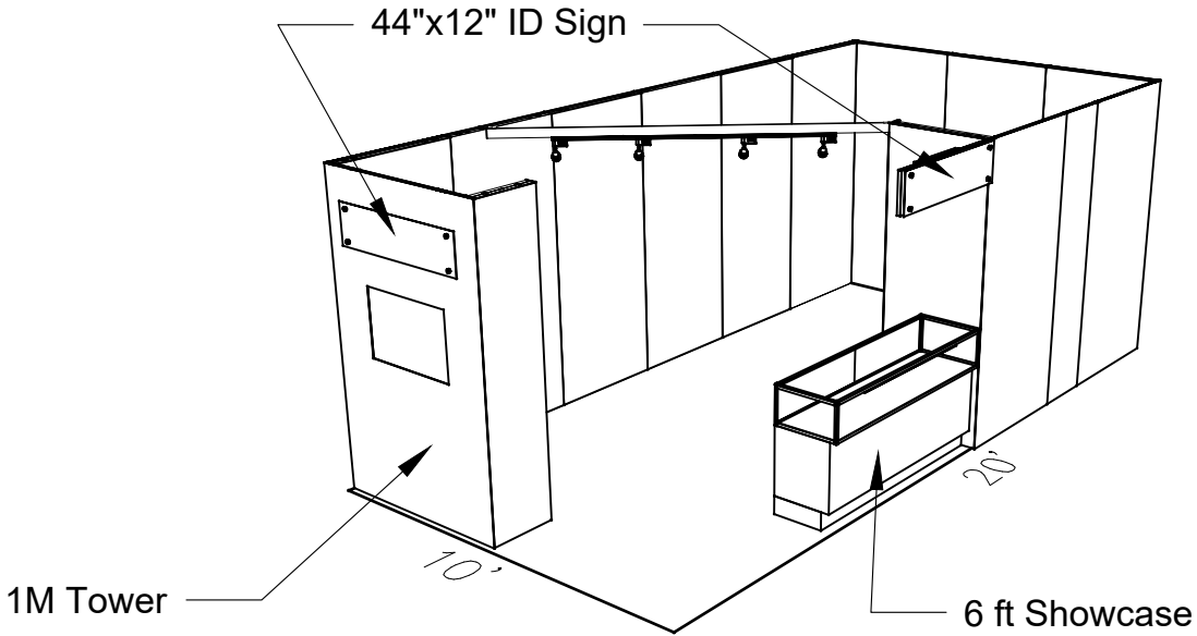
PERSPECTIVE - FRONT
