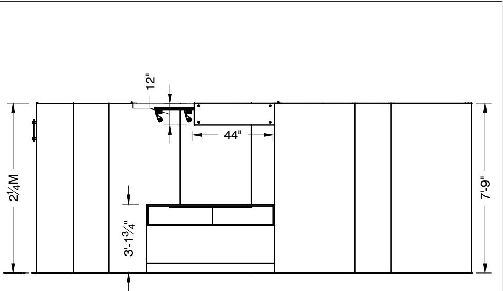
PLAN VIEW
