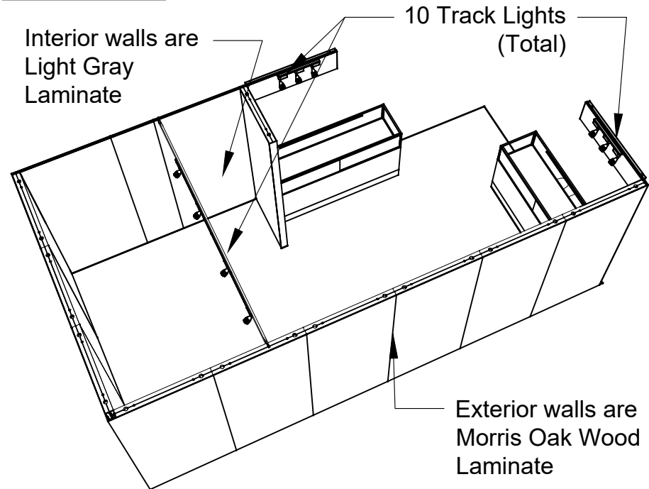
PERSPECTIVE - BACK
