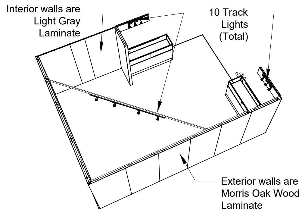
PERSPECTIVE - BACK
