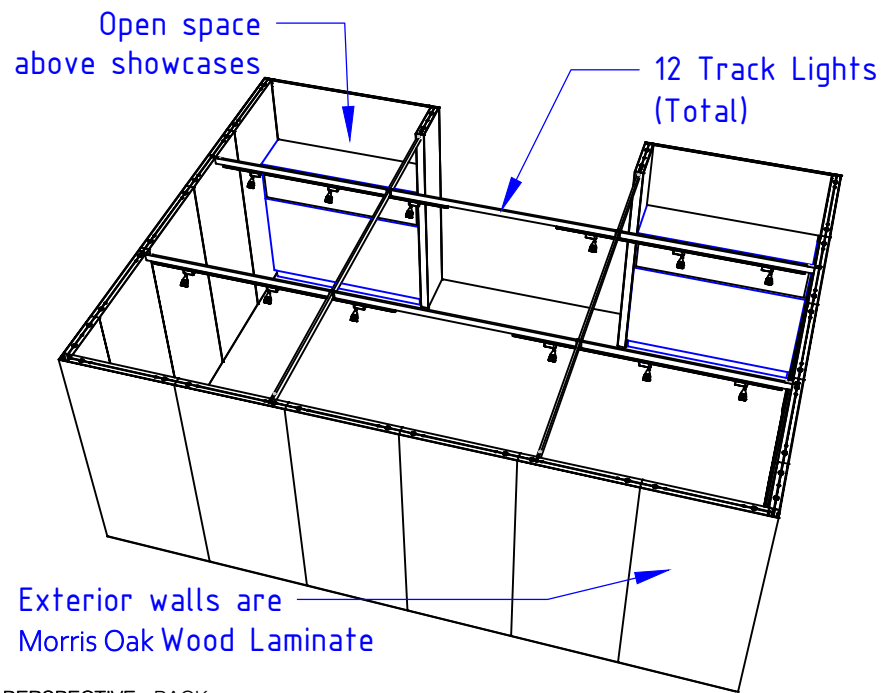
PERSPECTIVE - BACK
