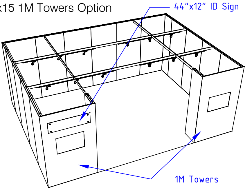
PERSPECTIVE - FRONT
