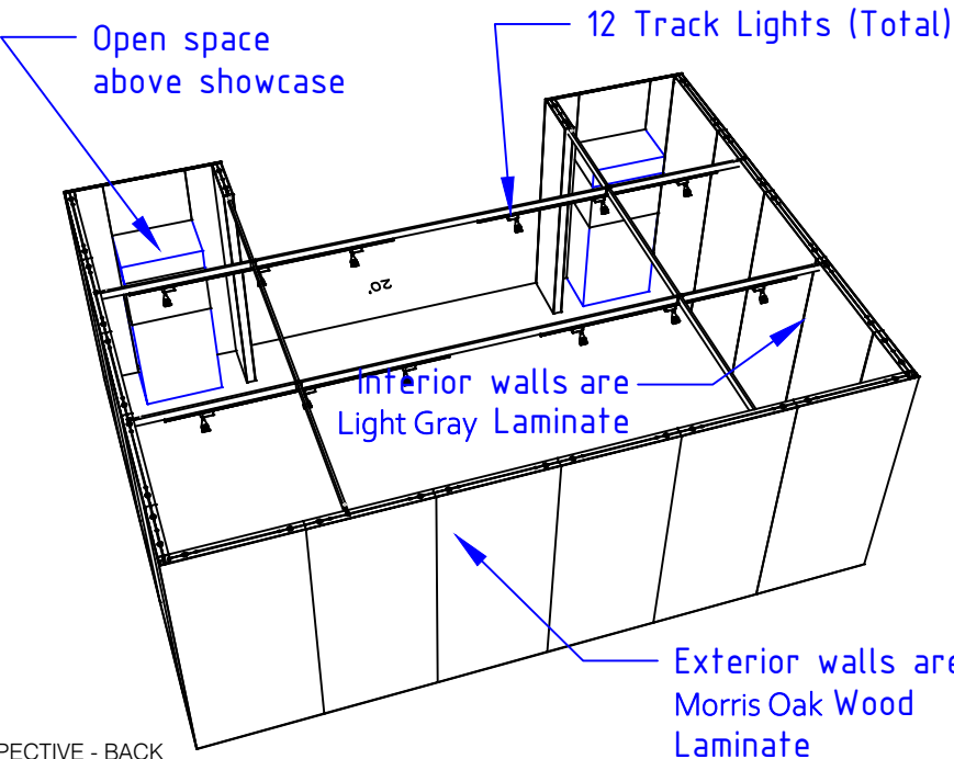
PERSPECTIVE - BACK
