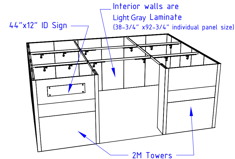
PERSPECTIVE - FRONT
