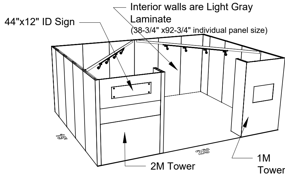
PERSPECTIVE - FRONT
