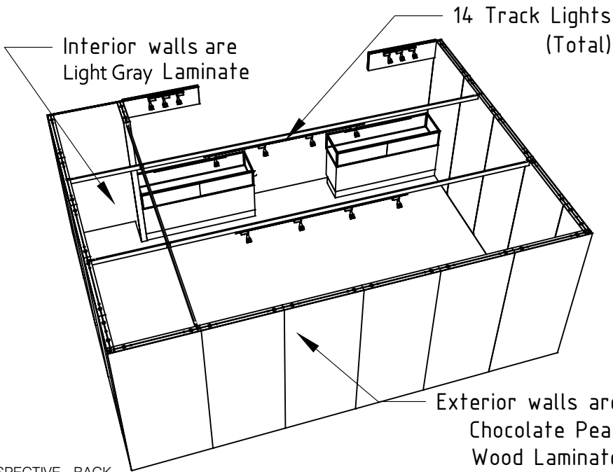
PERSPECTIVE - BACK
