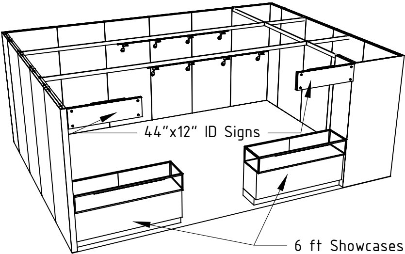
PERSPECTIVE - FRONT
