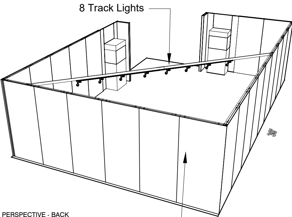
PERSPECTIVE - BACK
