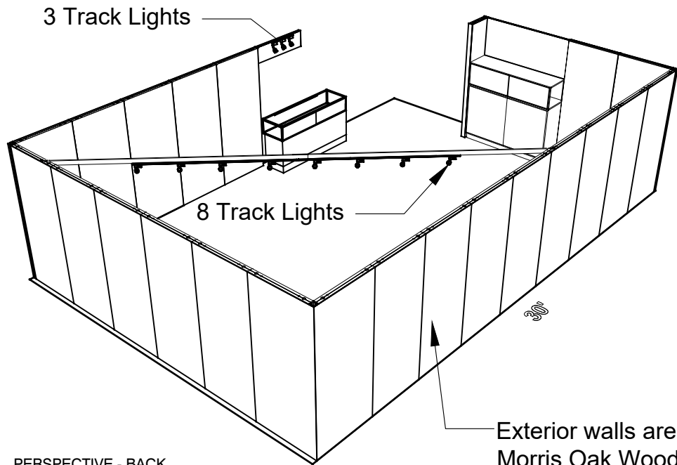
PERSPECTIVE - BACK
