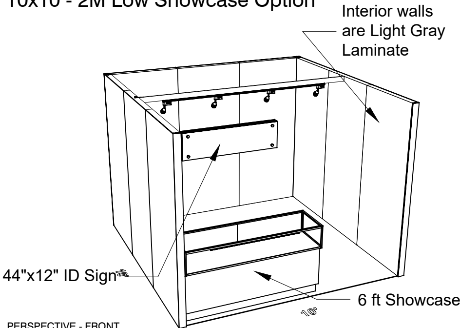
PERSPECTIVE - FRONT
