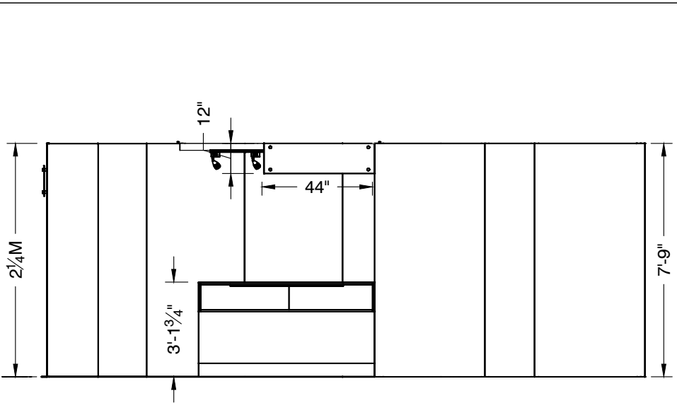
PLAN VIEW
