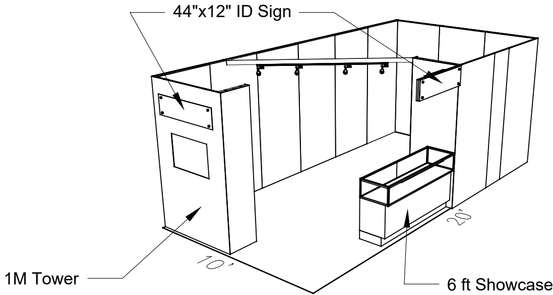
PERSPECTIVE - FRONT
