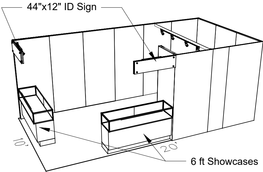
PERSPECTIVE - FRONT
