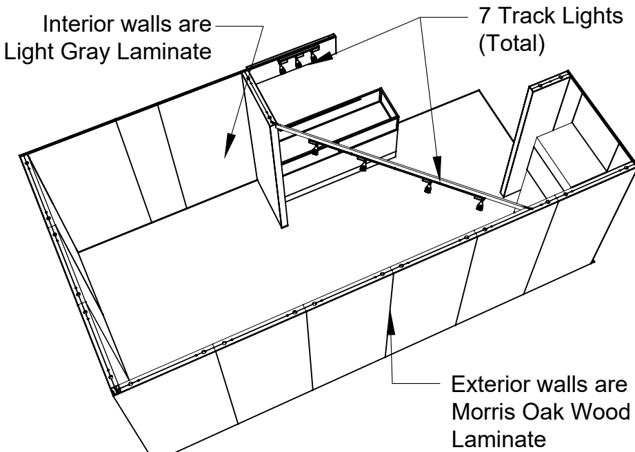
PERSPECTIVE - BACK
