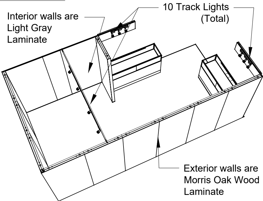
PERSPECTIVE - BACK
