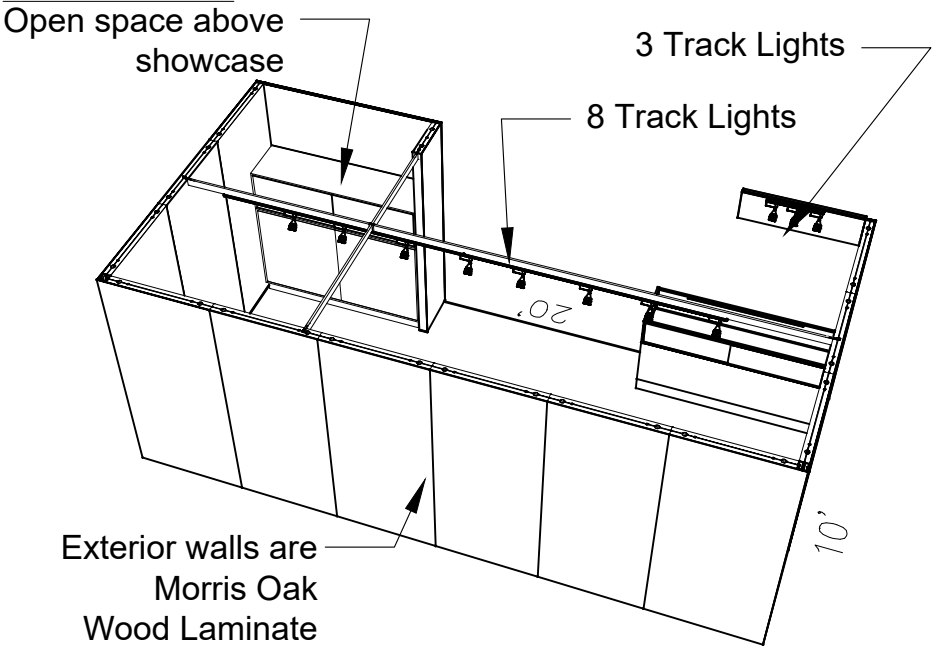
PERSPECTIVE - FRONT
