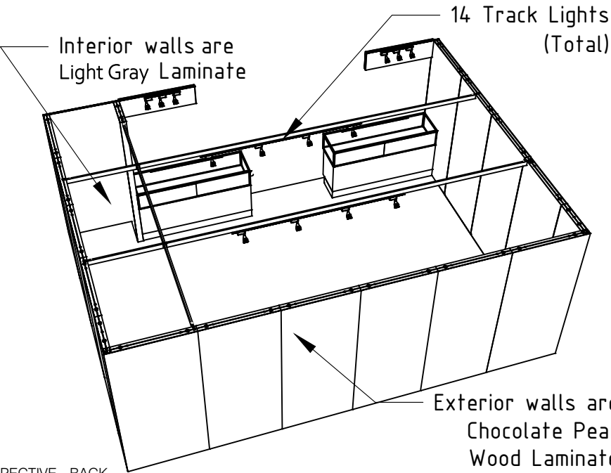
PERSPECTIVE - BACK
