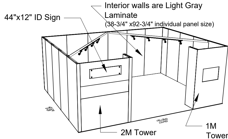
PERSPECTIVE - FRONT
