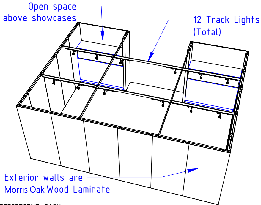
PERSPECTIVE - BACK
