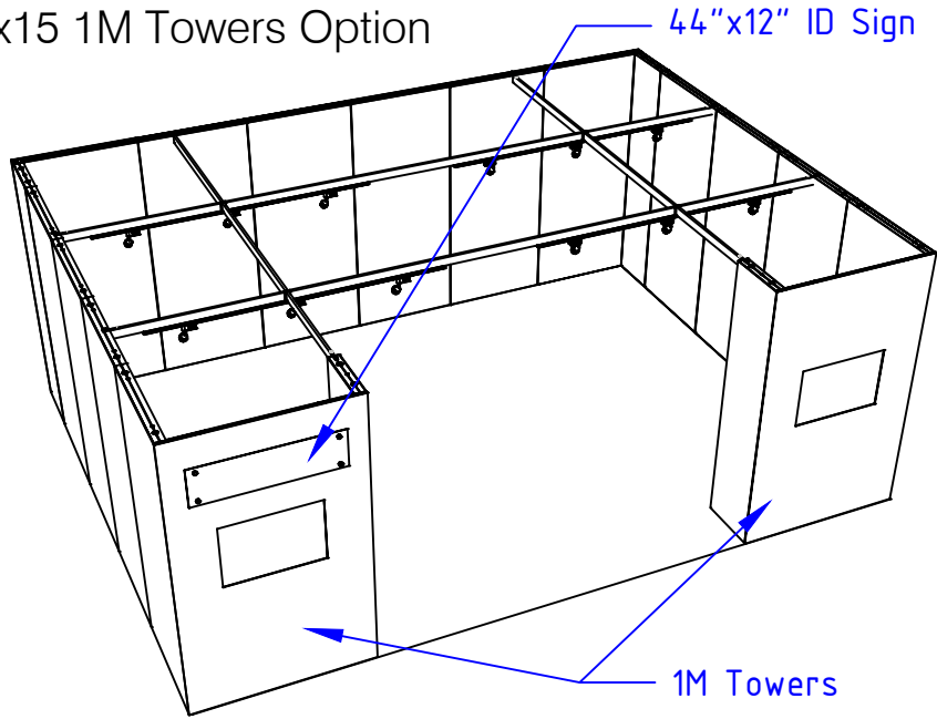
PERSPECTIVE - FRONT
