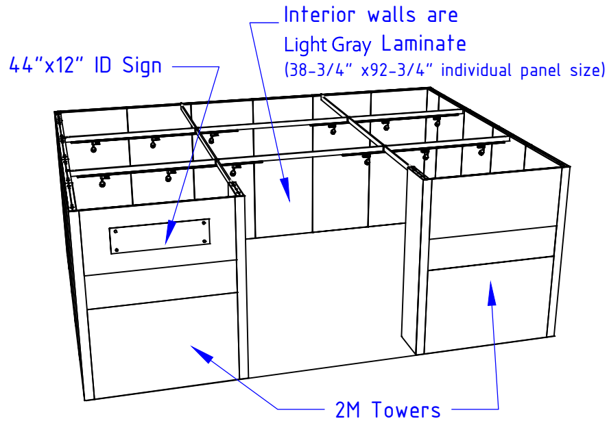
PERSPECTIVE - FRONT
