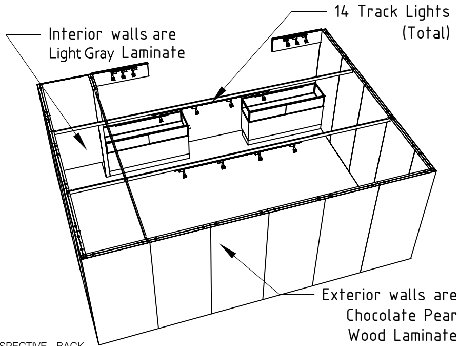
PERSPECTIVE - BACK
