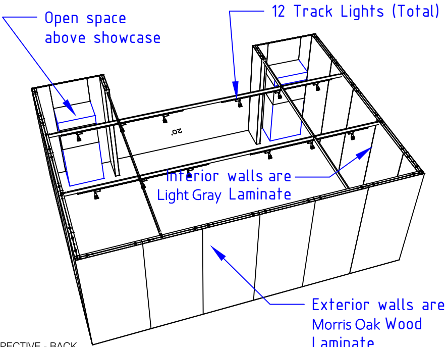
PERSPECTIVE - BACK
