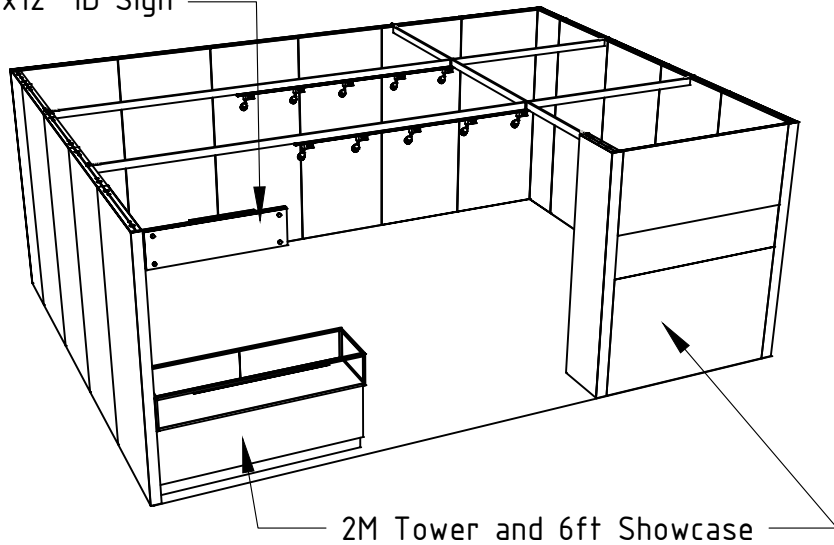
PERSPECTIVE - FRONT
