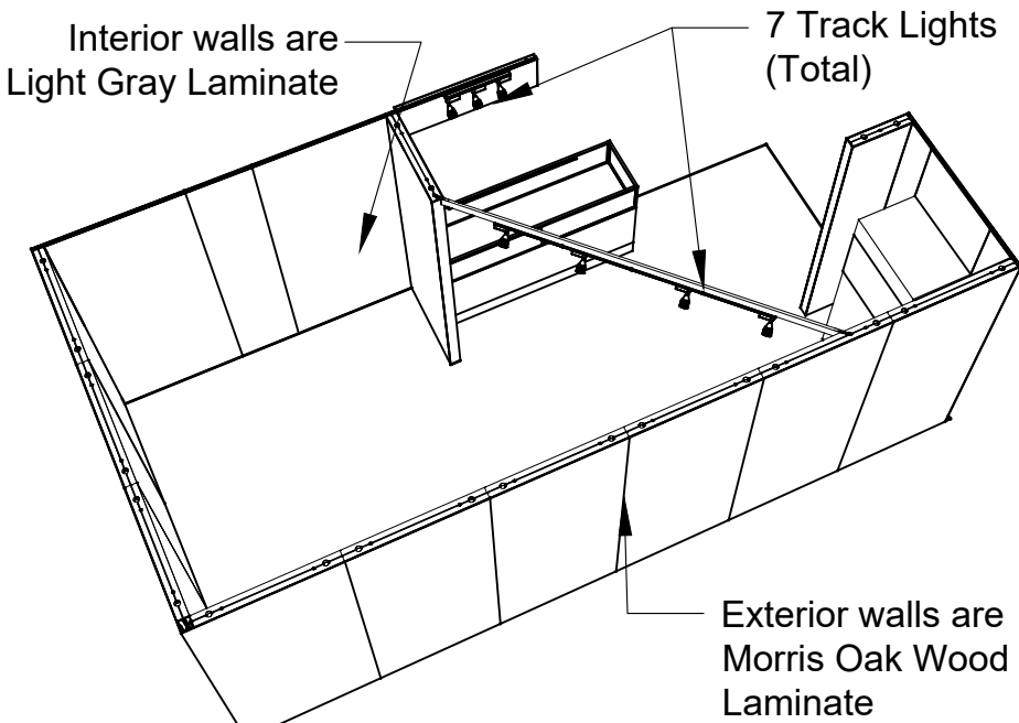
PERSPECTIVE - BACK
