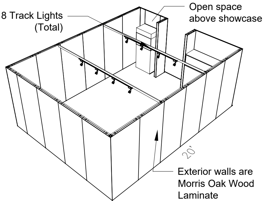
PERSPECTIVE - BACK
