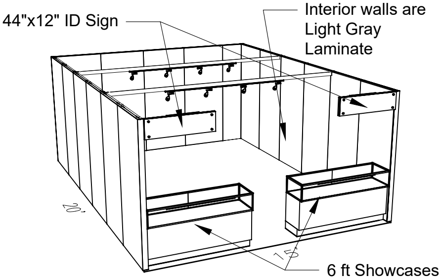
PERSPECTIVE - FRONT
