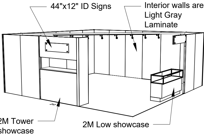
PERSPECTIVE - FRONT
