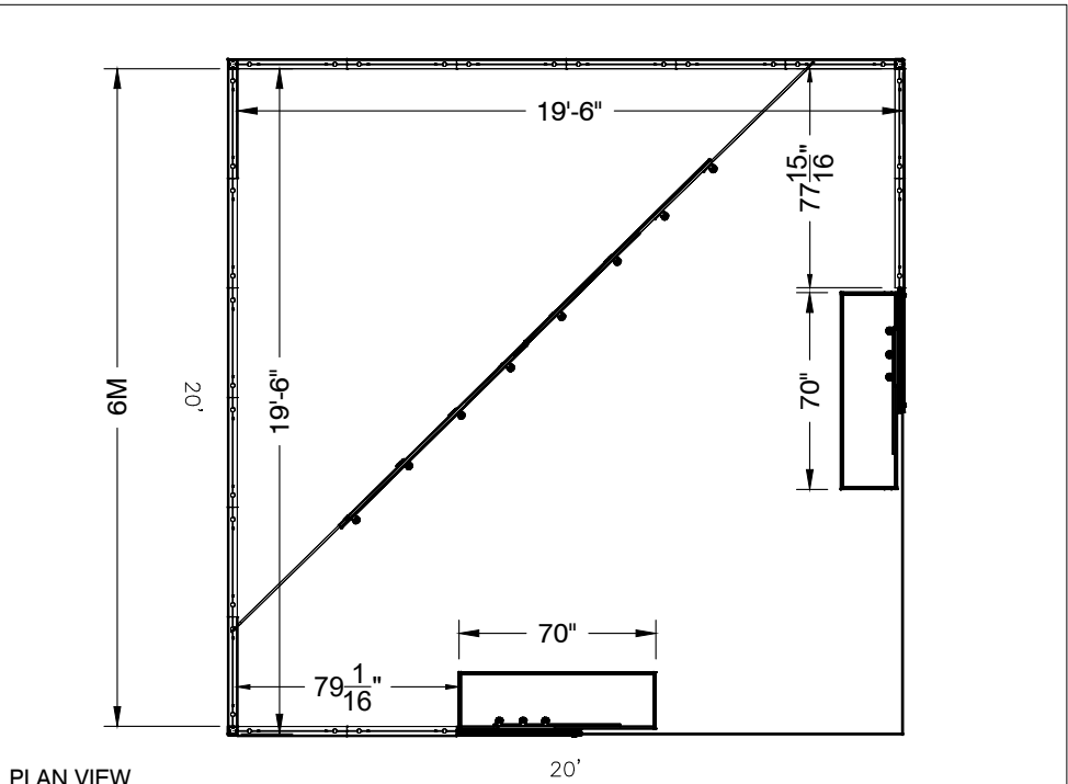
PLAN VIEW
