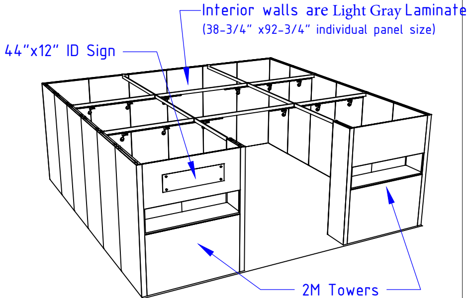
PERSPECTIVE - FRONT
